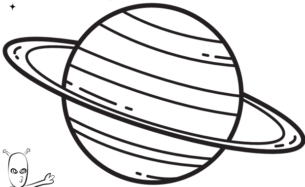
SATURN
